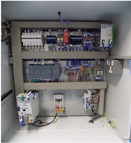
Control Panel Interior
